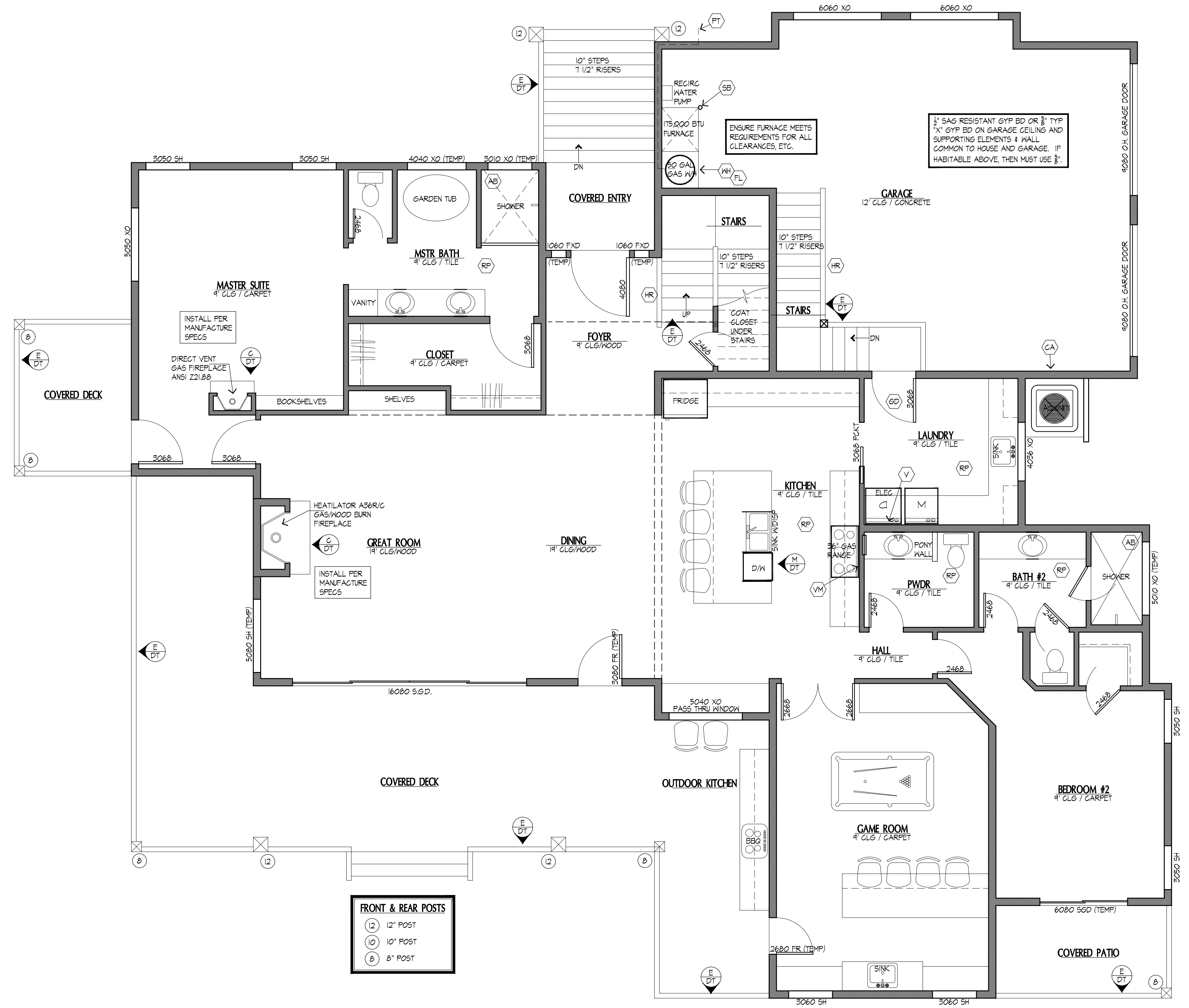
MAIN FLOOR PLAN GENERAL NOTES FOR THIS PAGE ARE ON THE GENERAL NOTES SHEET
