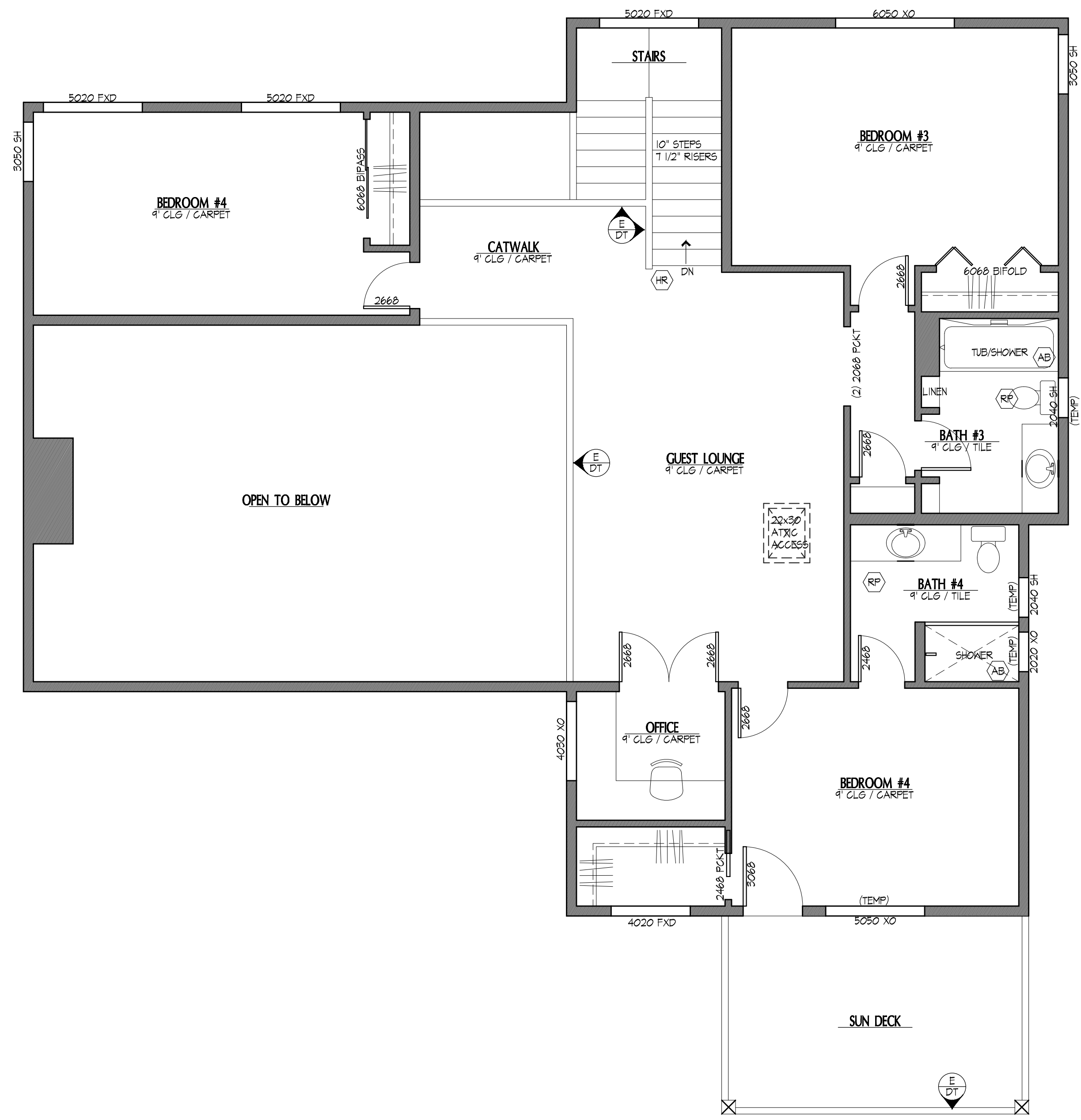
UPPER FLOOR PLAN GENERAL NOTES FOR THIS PAGE ARE ON THE GENERAL NOTES SHEET
