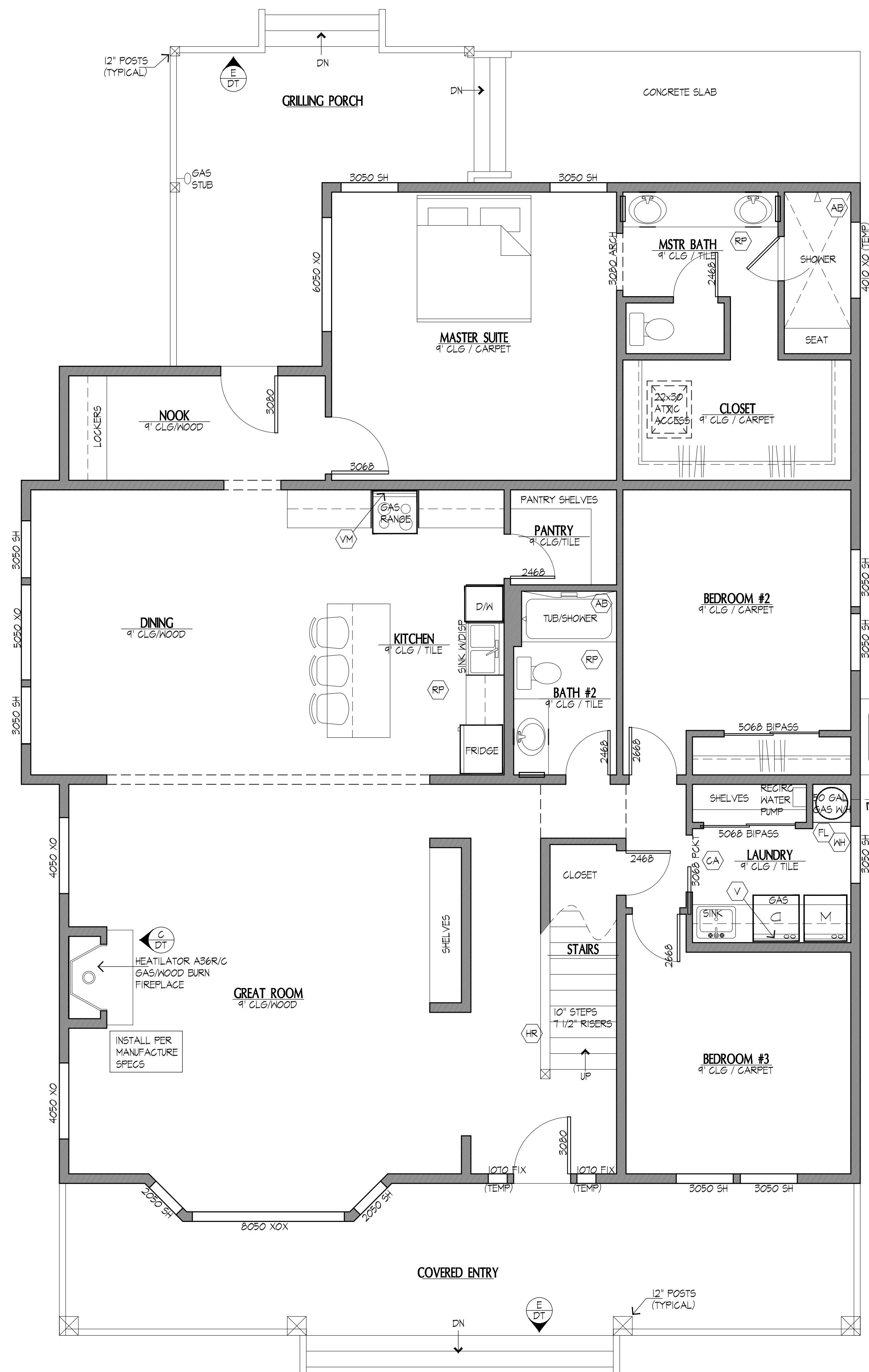
FLOOR PLAN GENERAL NOTES FOR THIS PAGE ARE ON THE GENERAL NOTES SHEET
